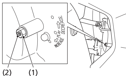
(2) clutch adjuster
