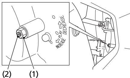
(2) clutch adjuster
