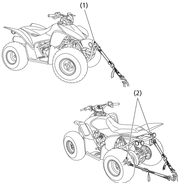
(1) front carry pipe (2) rear carry pipe or near axle shaft
